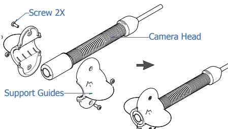
D80 Applicable to 4"-5" pipe.
