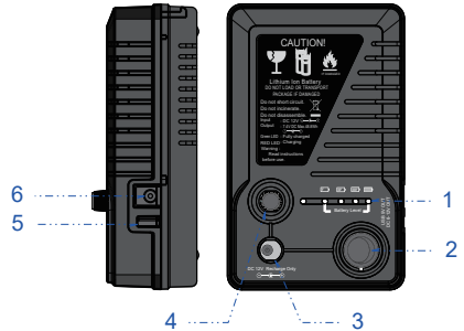
Figure 4. Battery pack
